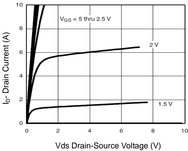
V GS = 5 thru 2.5 V Figure 5 Output CHARACTERISTICS
