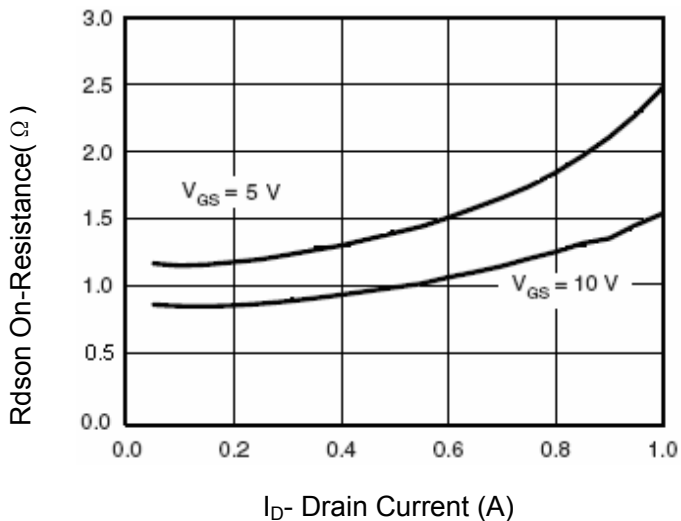
Figure 5 Drain-Source On-Resistance
