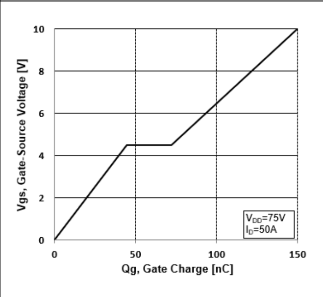
Figure 13. Typical Gate Charge vs Gate-Source Voltage
