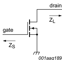
Fig 6. Definition of transistor impedance
