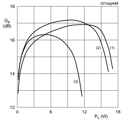
V_{DS} = 32\text{ V}; I_{Dq} = 25\text{ mA}; t_p = 100\text{ }\mu\text{s}; \delta = 20\text{ }\% (1) f = 2.7\text{ GHz} (2) f = 2.9\text{ GHz} (3) f = 3.1\text{ GHz}
