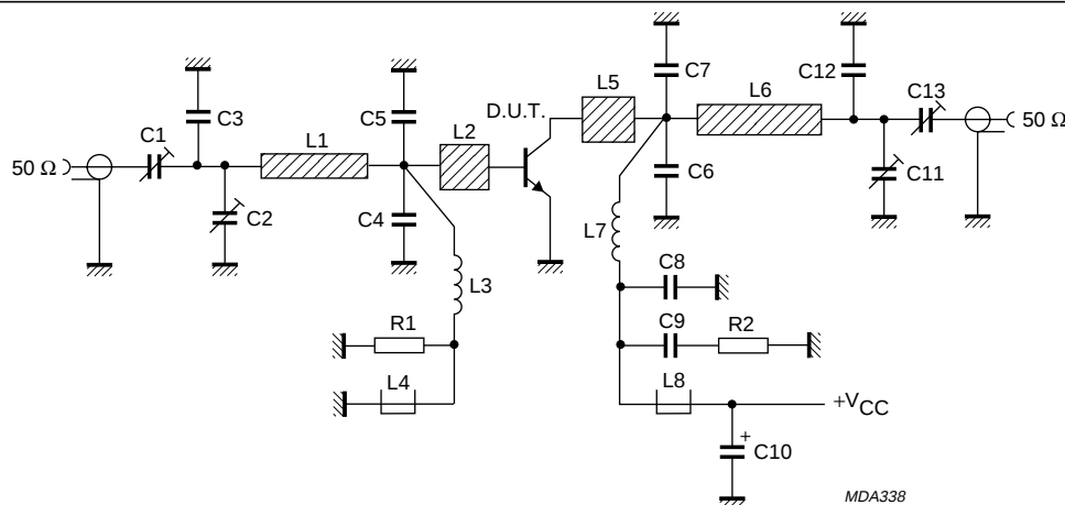
Fig.5 Class-B test circuit at f = 470\text{ MHz} .
