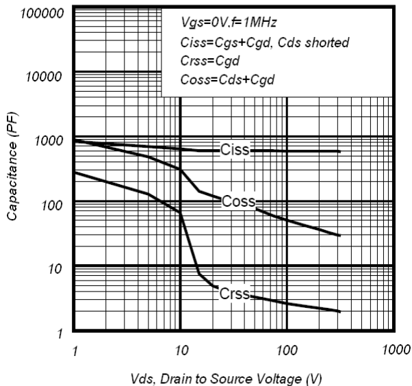
Fig 8. Capacitance Characteristics
