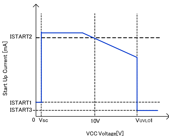
Figure 5. Startup Current vs VCC Voltage (*Startup current flows from the VH pin.)
