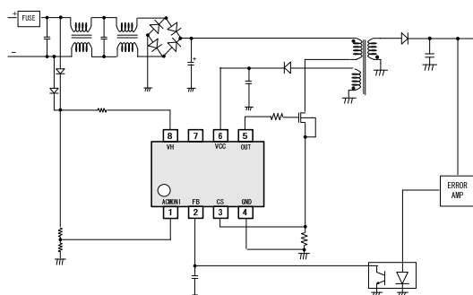
Figure 1. Application Circuit
