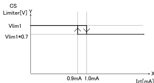
Figure 20 Izt Current vs Switched CS Voltage Characteristics
