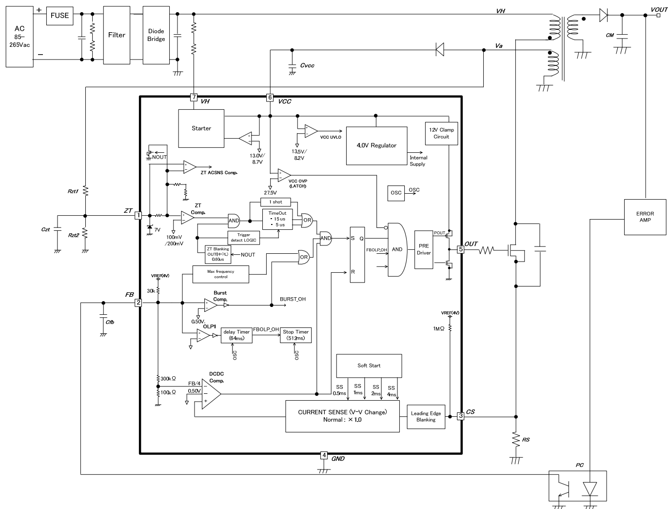
Figure 4. Block Diagram
