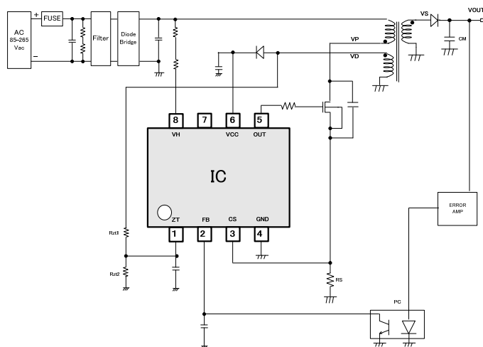
Figure 1. Application Circuit
