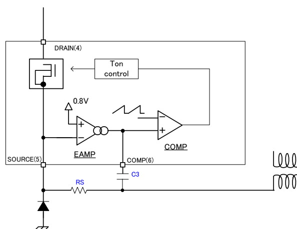
Figure 11. Diagram of error amplifier block
