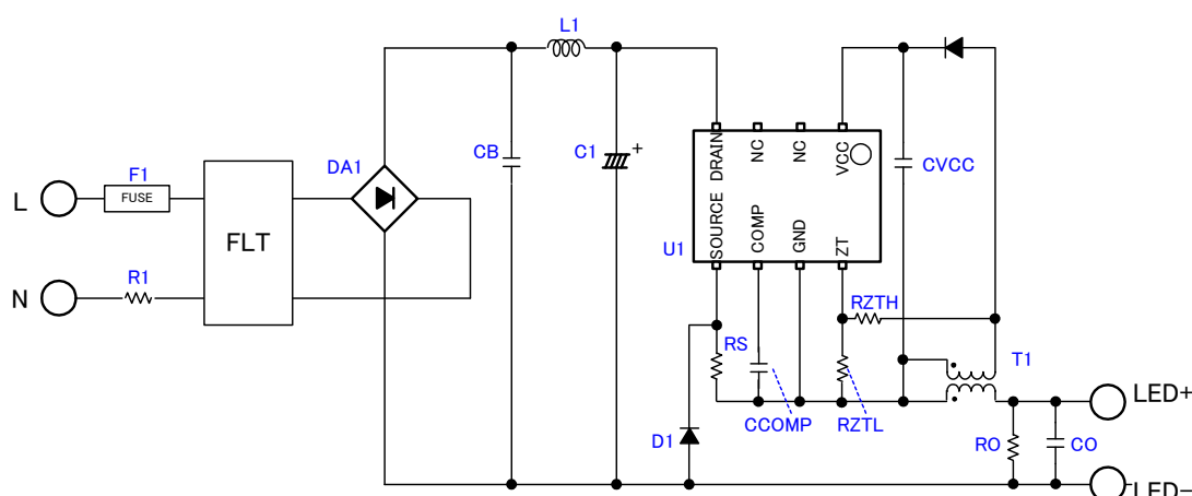
Figure 1. Application circuit
