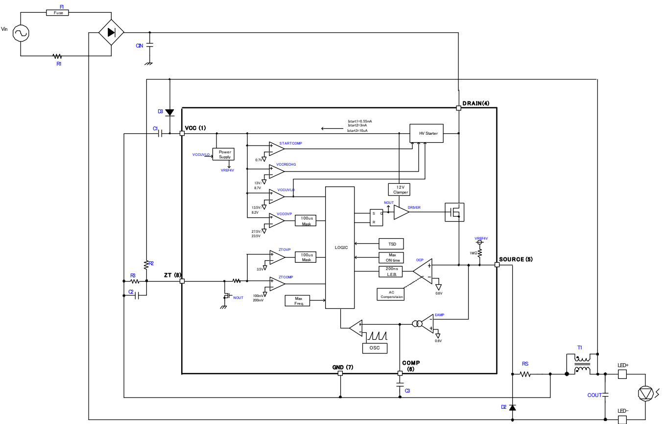
Figure 3. Block diagram
