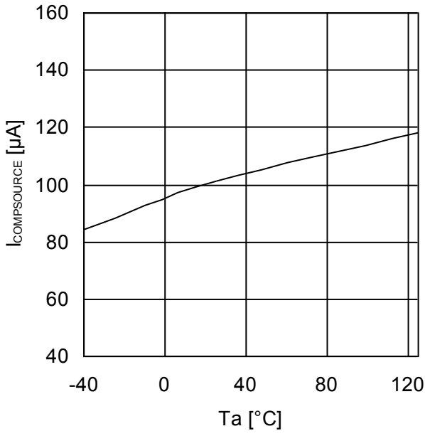
Figure 11. COMP Pin Source Current
