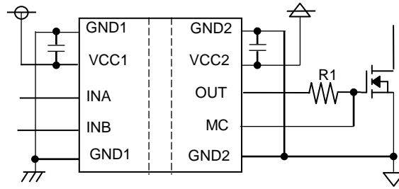
Figure 31. Driving SiC
