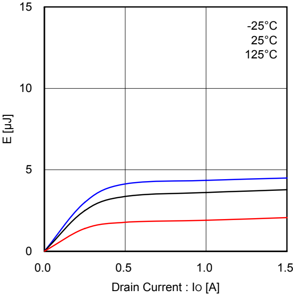
Fig.35 Low side recovery loss (VDC=300V)
