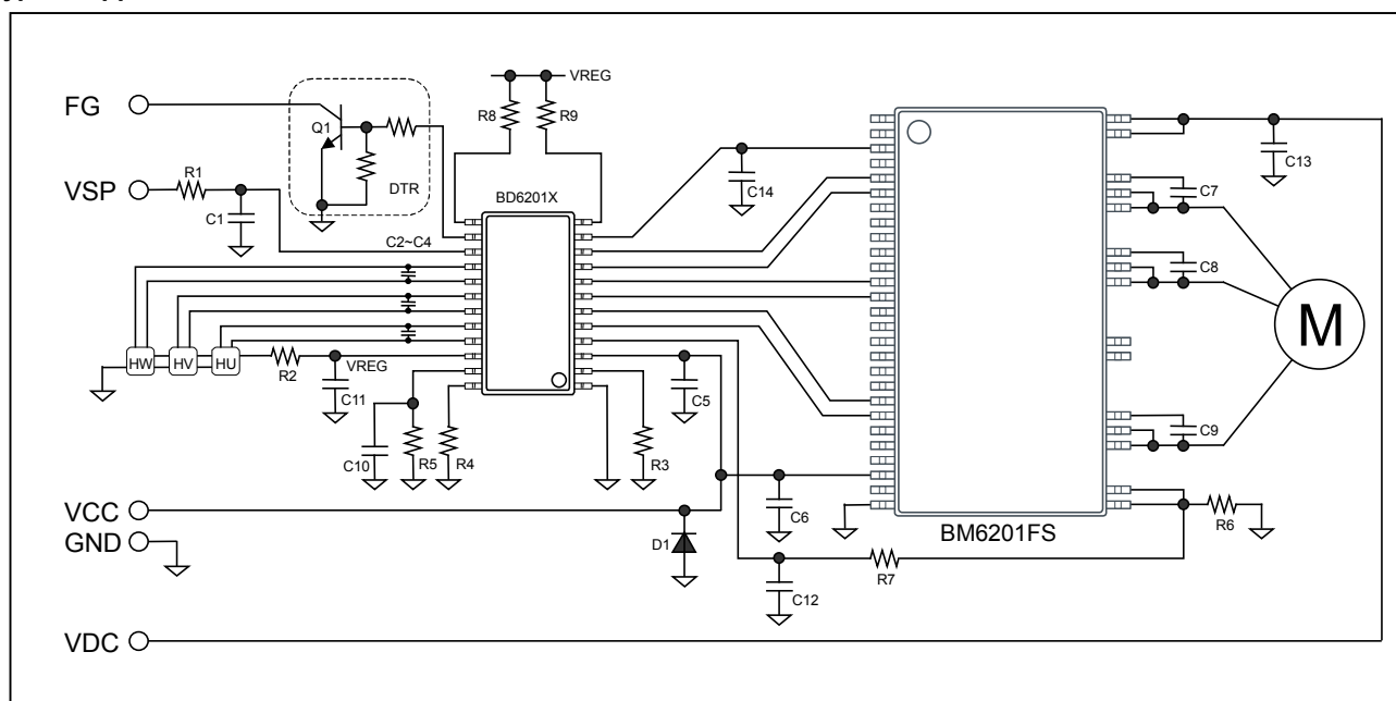
Fig.1 Application circuit example - BM6201FS &amp; BD6201X
