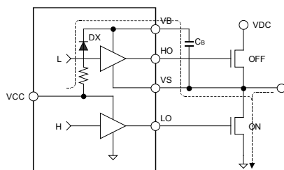
Fig.5 Charging period
