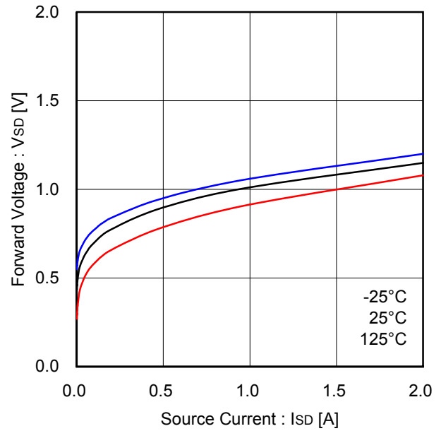
Fig.29 Output MOSFET body diode
