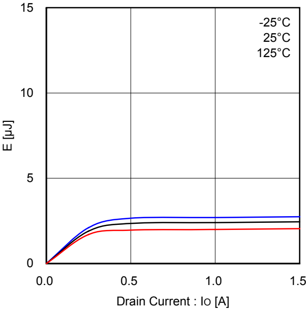
Fig.33 High side recovery loss (VDC=300V)
