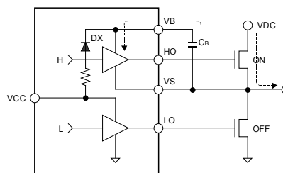
Fig.6 Discharging period
