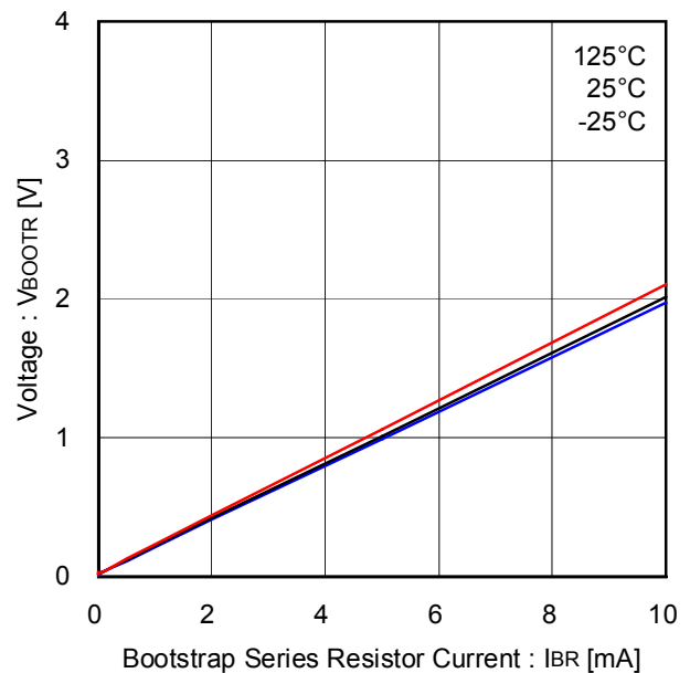
Fig.31 Bootstrap series resistor
