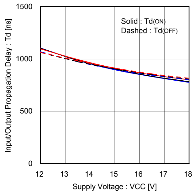
Fig.27 Input/Output propagation delay
