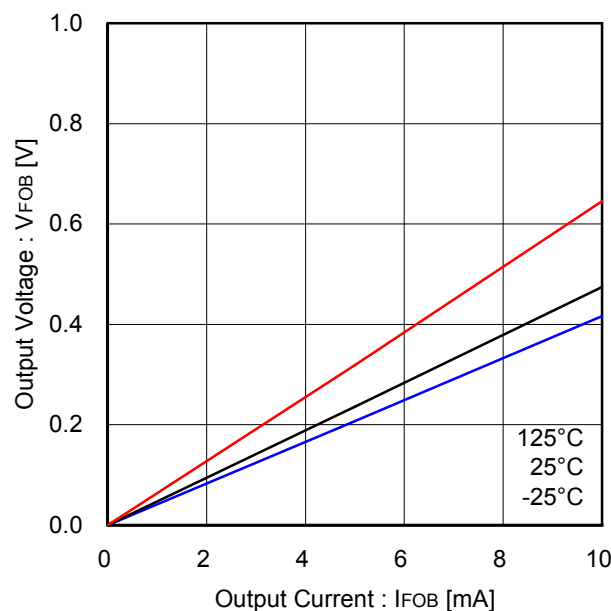
Fig.23 Fault output on resistance
