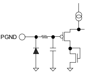
Fig.38 PGND
