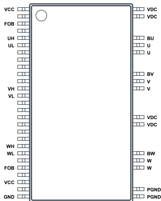
Fig.3 Pin configuration
