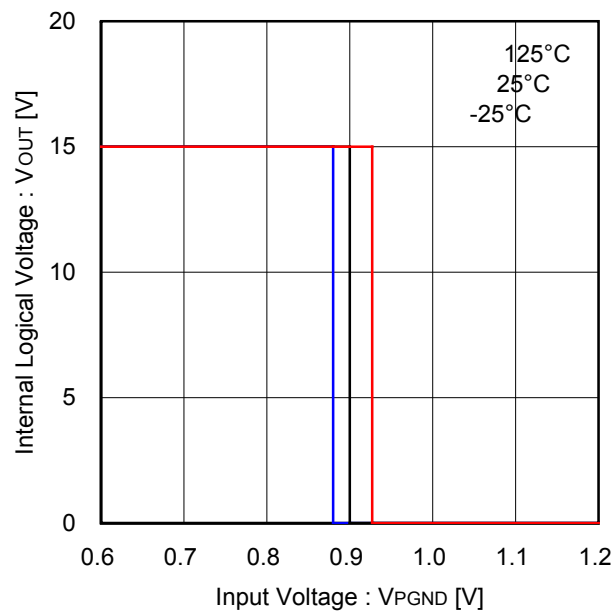
Fig.19 Overcurrent detection voltage
