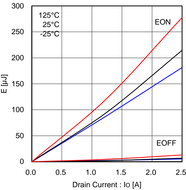
Figure 33. High Side Switching Loss (VDC=300V)
