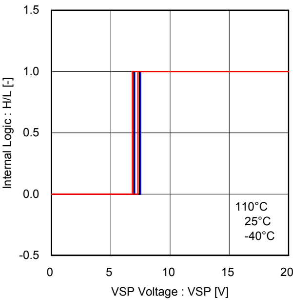
Figure 32. Testing Mode Threshold Voltage
