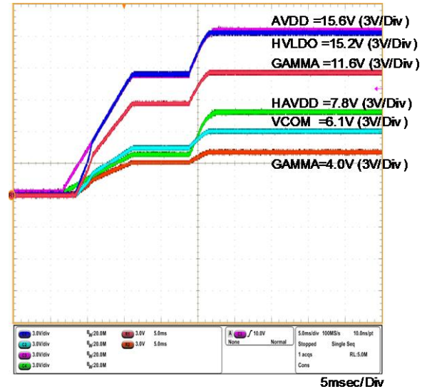
Figure 8. Power-on (after AVDD on)
