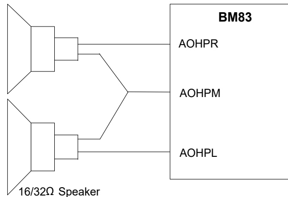
Figure 3-30. Analog Speaker Output - Capless Mode
