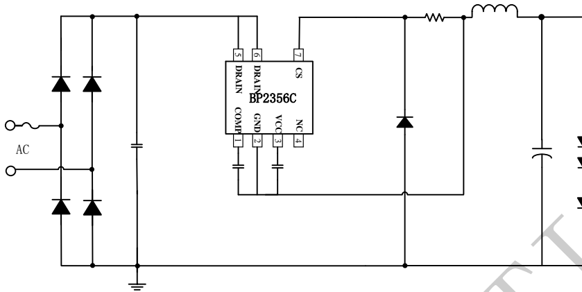
Figure 1. Typical application circuit without OVP for BP2356C
