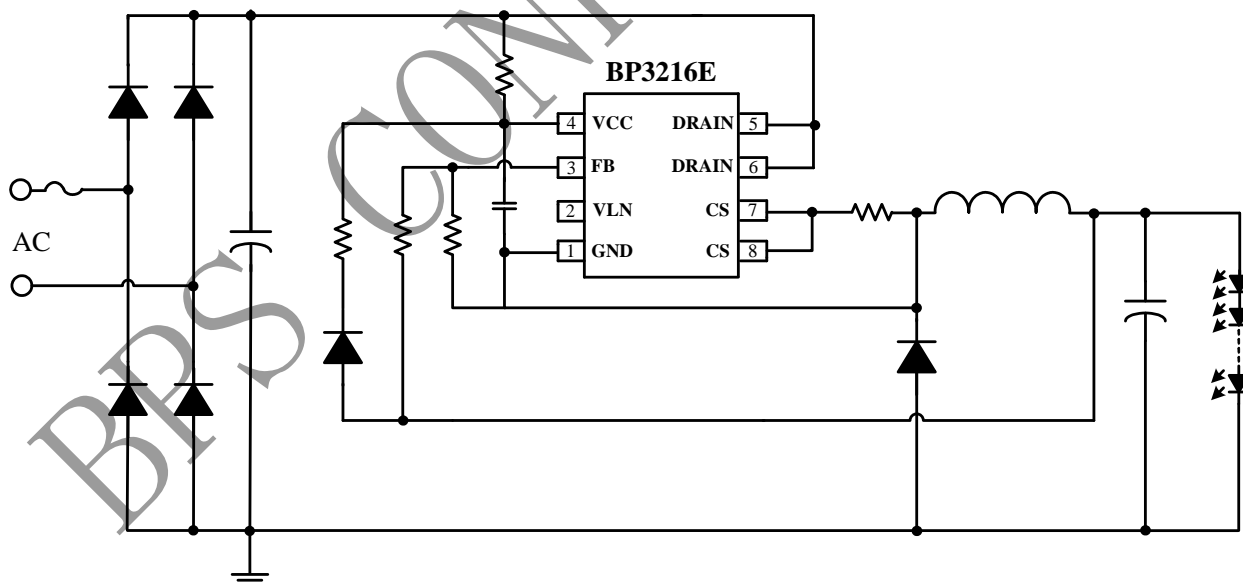
Figure 1. Typical application circuit for BP3216E (Buck)
