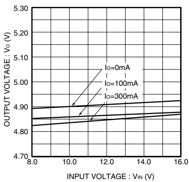
Fig.5 Line regulation
