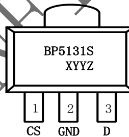
Fig 2 BP5131S Pin Mapping
