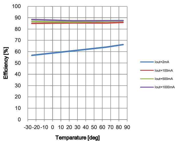
Fig.20-2 Temperature Characteristics (Vout:BP5293-12)
