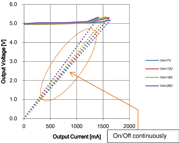
Fig.16 Over Current Limit (Vout : BP5293-50)
