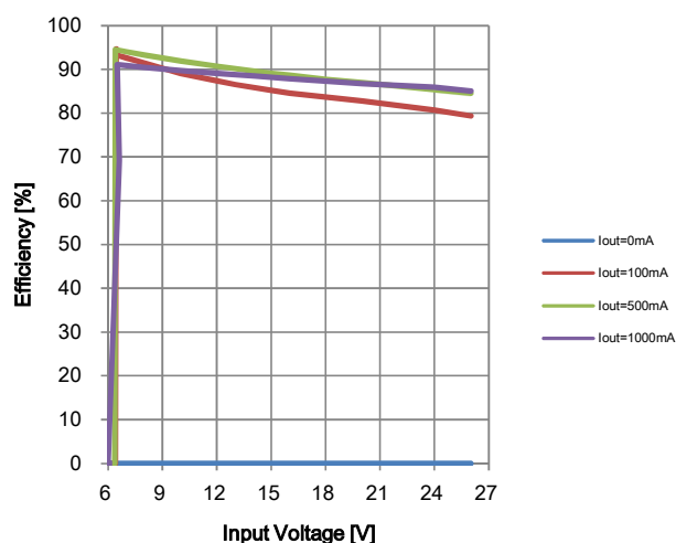
Fig.13-2 LINE Regulation (Efficiency : BP5293-50)
