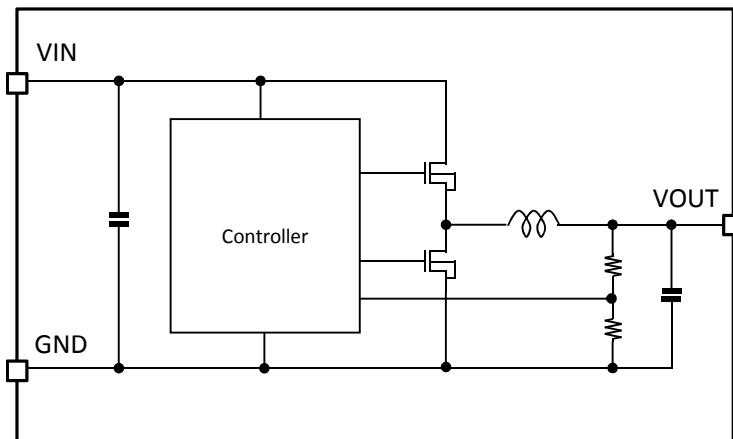
Fig.3 Block diagram
