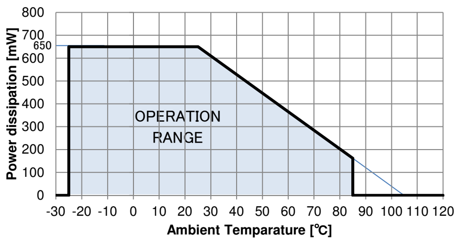
Fig.23 Power dissipation
