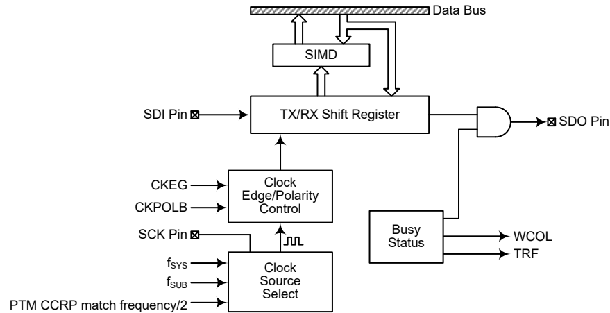
SPI Master Mode Block Diagram
