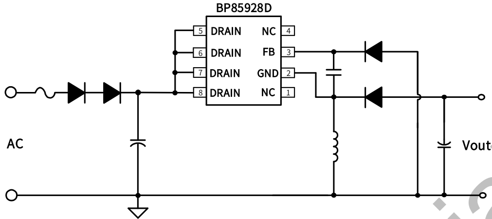
Figure2. Typical buck-boost application with the BP85928D
