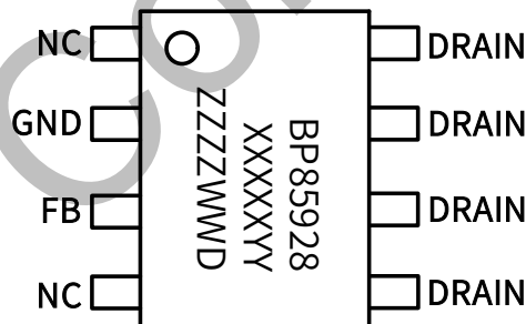
Figure 3. SOP-8 pin configuration
