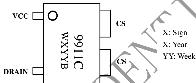
Figure 2. Pin configuration
