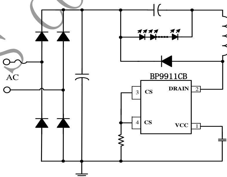
Figure 1. Typical application circuit for BP9911CB
