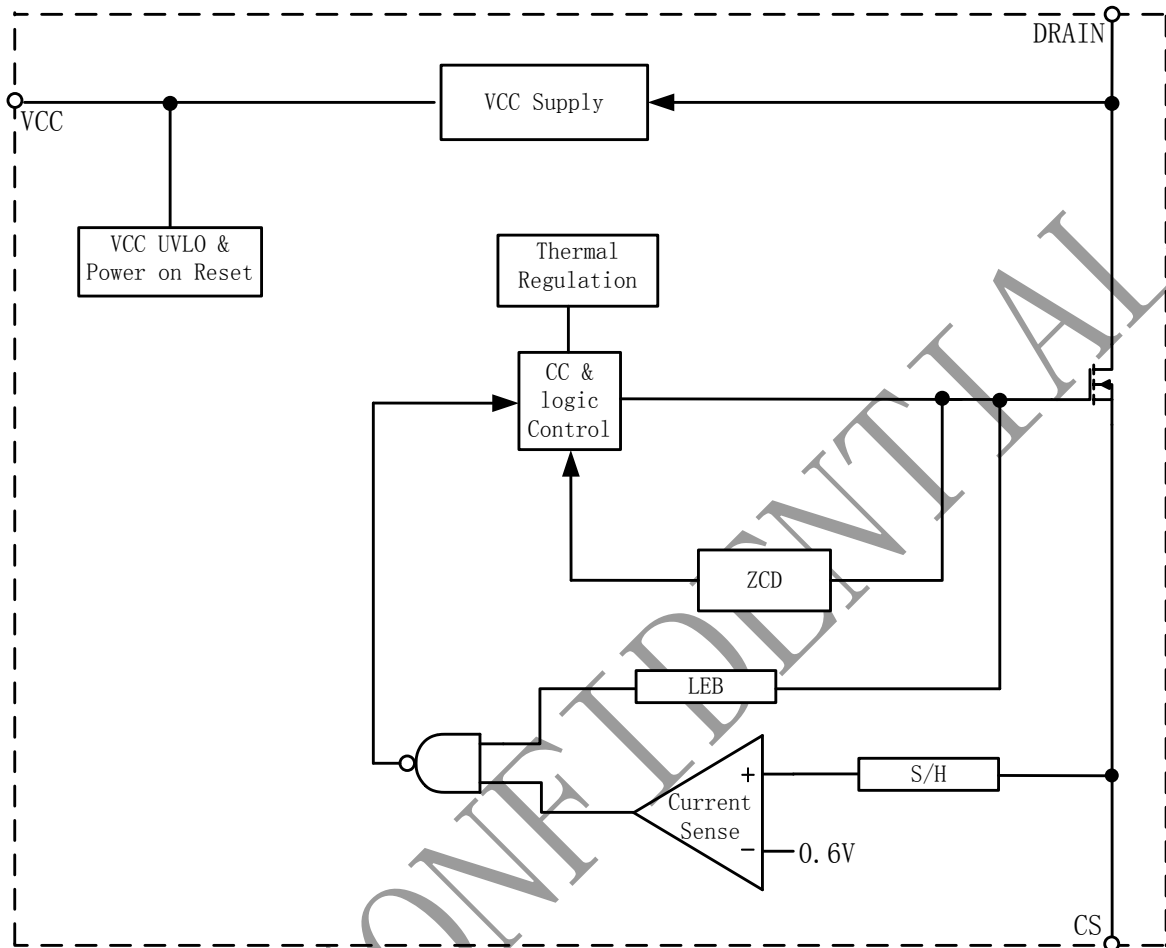
Figure 3. BP9912CB Internal Block Diagram
