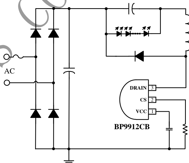
Figure 1. Typical application circuit for BP9912CB
