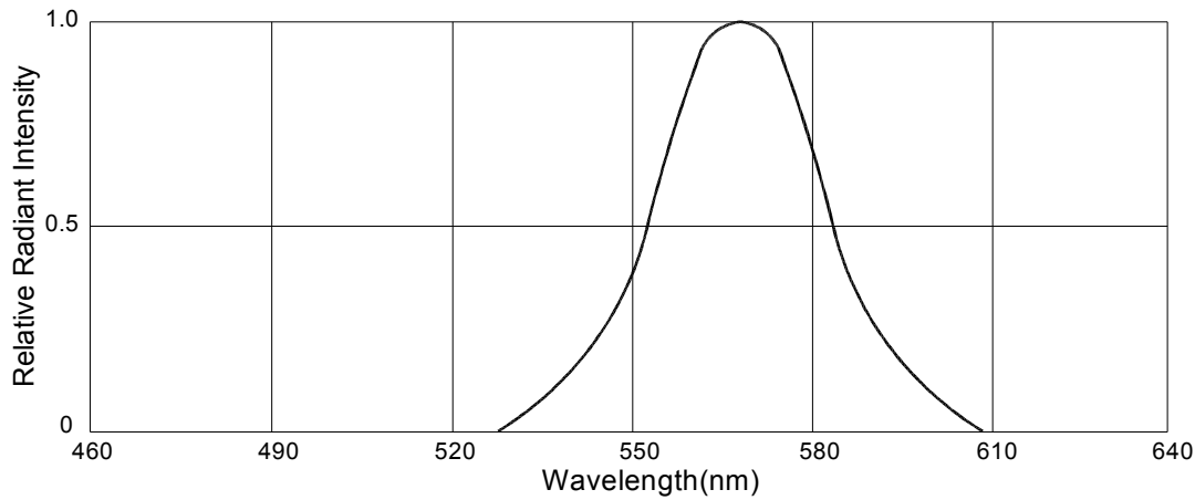
Fig.1 Relative Radiant Intensity VS. Wavelength
