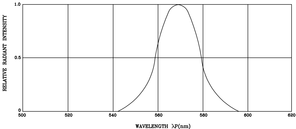
SPECTRAL DISTRIBUTION
