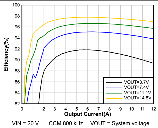
Figure 8-4. System Efficiency
