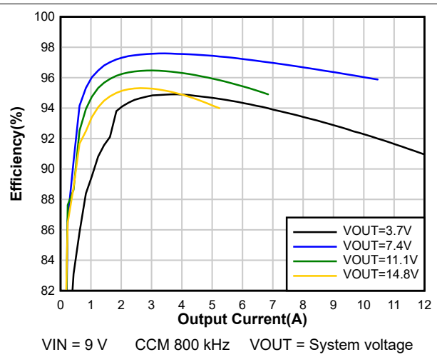
Figure 8-2. System Efficiency
