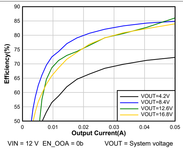
Figure 8-6. Light Load System Efficiency
