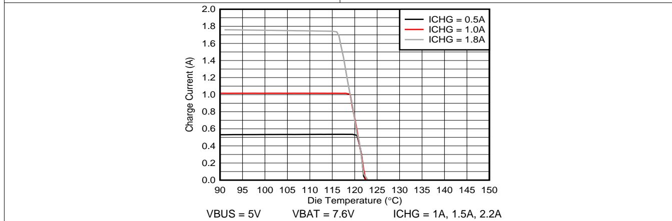
Figure 17. Max Current Temperature Profile
