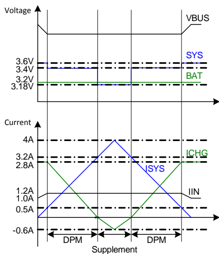
Figure 11. DPM Response
