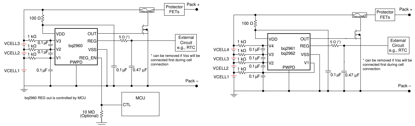
Figure 16. Application Schematic
