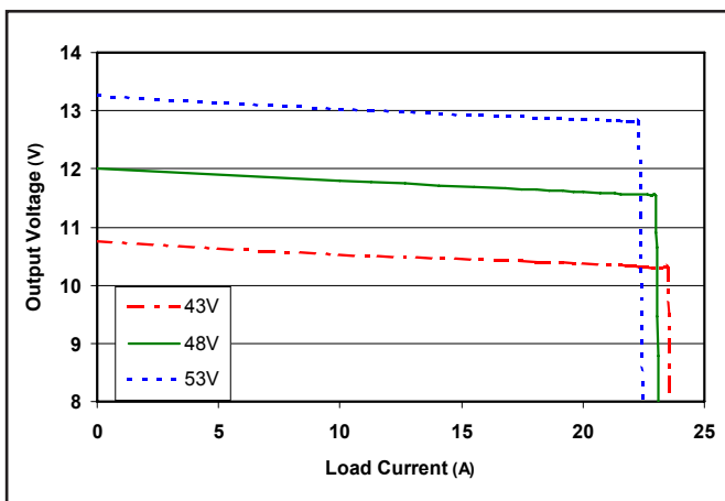
Figure 16: Output voltage vs. load current showing typical current limit curves and converter shutdown points.
