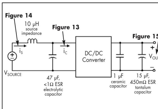
Figure 12: Test set-up diagram showing measurement points for Input Terminal Ripple Current (Figure 13), Input Reflected Ripple Current (Figure 14) and Output Voltage Ripple (Figure 15).
