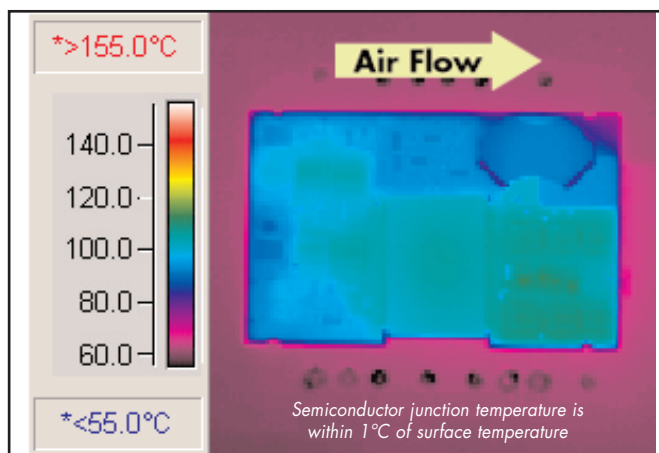
Figure 8: Thermal plot of converter at 20 amp load current (240W) with 55°C air flowing at the rate of 200 LFM. Air is flowing across the converter from input to output (nominal input voltage).
