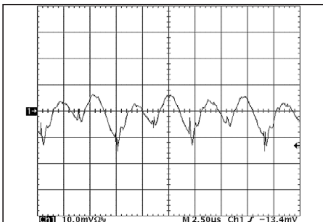
Figure 14: Input reflected ripple current, i_S , through a 10\mu\text{H} source inductor at nominal input voltage and rated load current (5 mA/div). See Figure 12.
