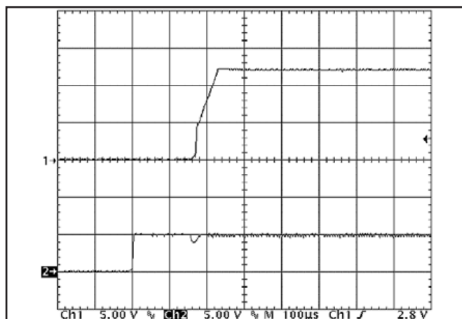
Figure 10: Turn-on transient at zero load (100 μs/div). Top Trace: V_{out} (5V/div) Bottom Trace: ON/OFF input (5V/div)
