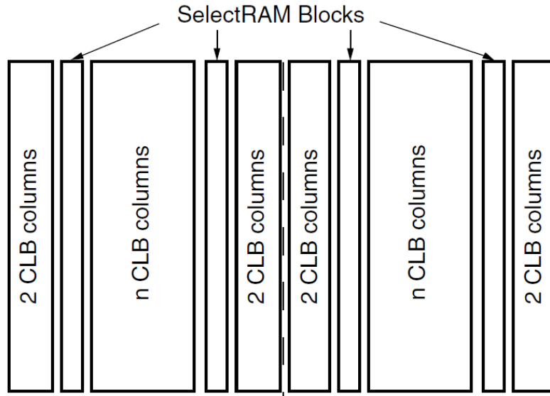
Figure 27 Block SelectRAM(4-column)
