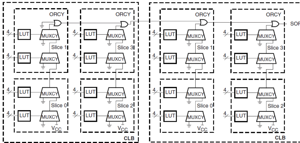
Figure 18 Horizontal Cascade Chain
