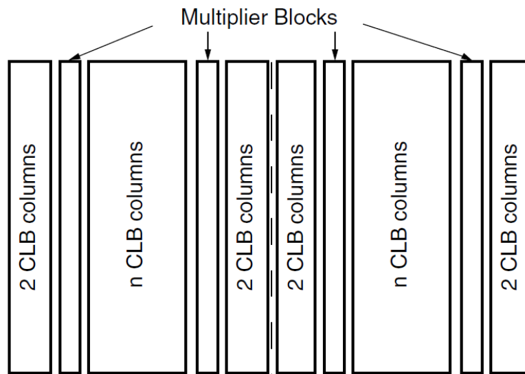
Figure 30 Multipliers(4-column)
