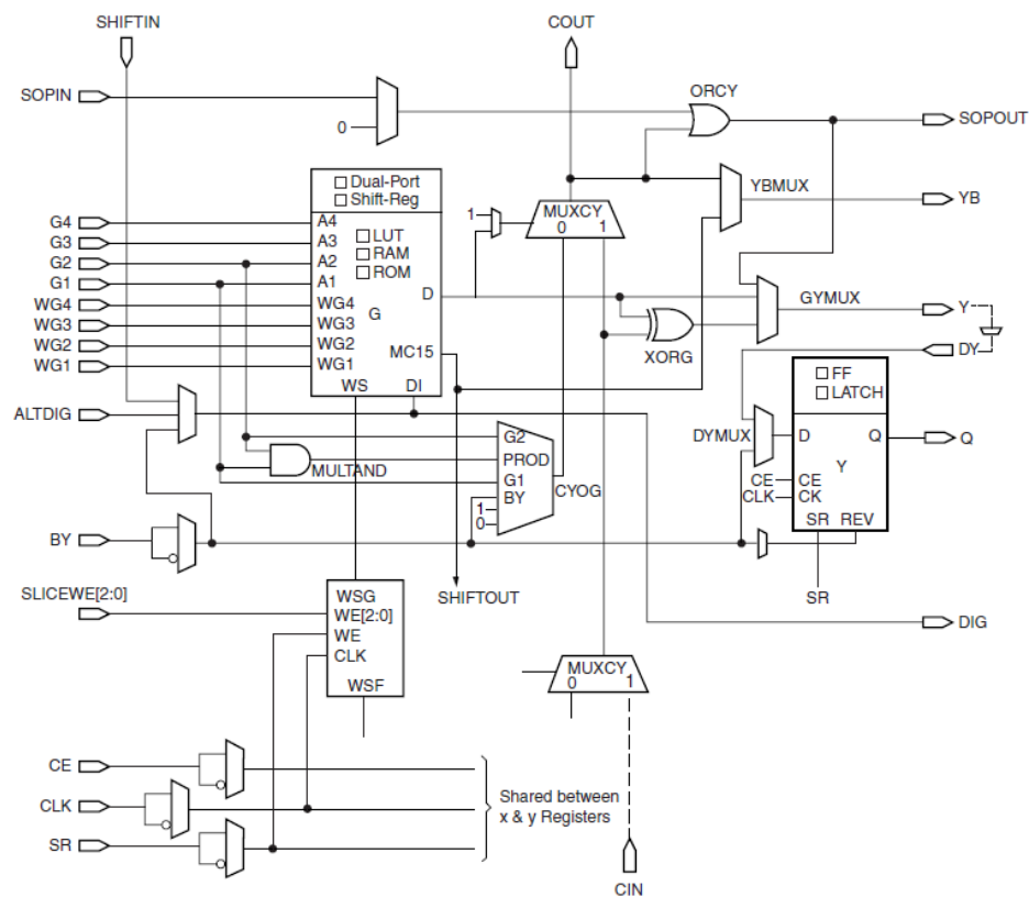
Figure 11 BQR2V6000 Slice(Top Half)
