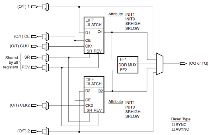
Figure 5 Register/Latch Configuration in an IOB Block
