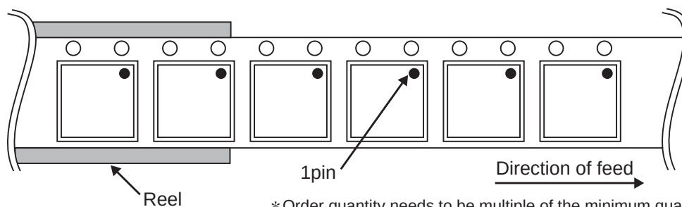
Tape Embossed carrier tape Quantity 4000pcs Direction of feed TR ( The direction is the 1pin of product is at the upper right when you hold reel on the left hand and you pull out the tape on the right hand )
