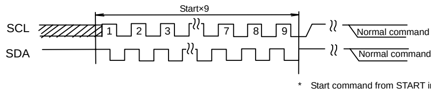
Figure 47-(c) START x 9 + command input
