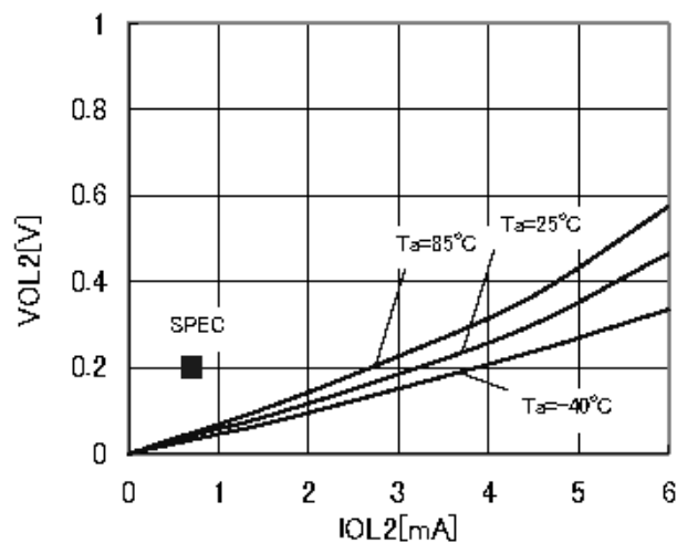
Figure 5. "L" Output Voltage2 VOL2-IOL2 ( V_{CC}=1.8V )
