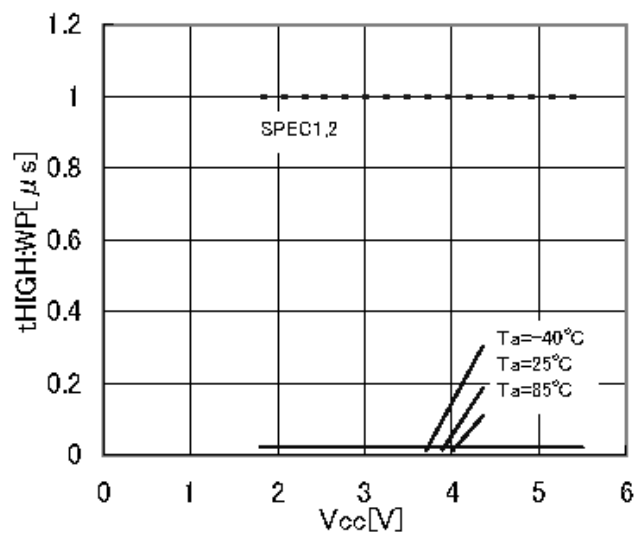
Figure 33. WP valid time t_{HIGH:WP}
