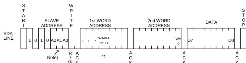
Figure 35. Byte write cycle (BR24L01A/02/04/08/16-W)
