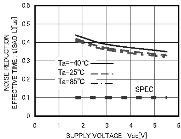
Figure 28. Noise reduction effective time t_I(\text{SDA L})
