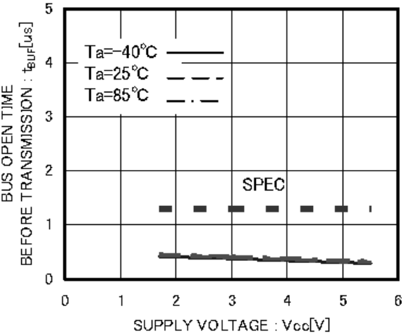
Figure 23. BUS open time before transmission tBUF
