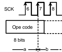
Figure 48. WREN/WRDI cancel valid timing
