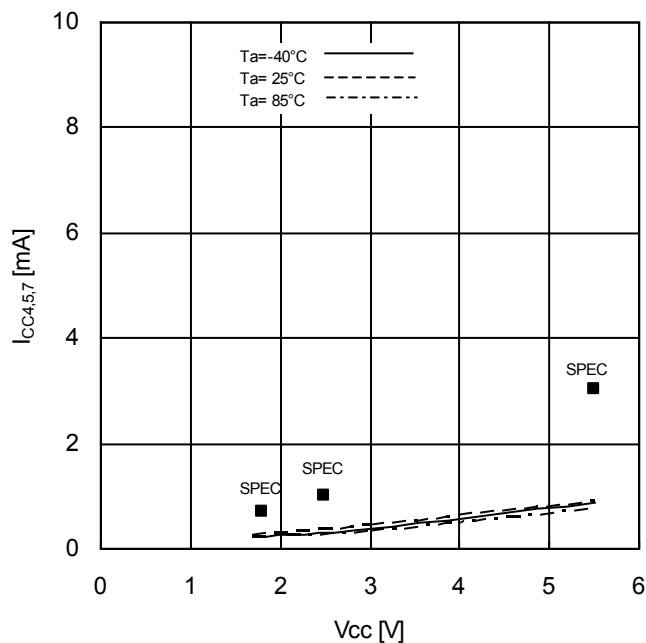
Figure 16. Supply Current (Read) vs Supply Voltage ( f_{SCK}=5\text{MHz} )
