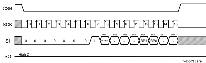
Figure 40. Write status register
