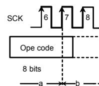
Figure 47. WREN/WRDI cancel valid timing
