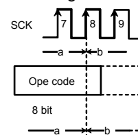
Fig.50 WREN/WRDI cancel valid timing
