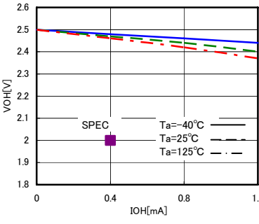
Fig.9 "H" output voltage V_{OH-IOH}(V_{CC}=2.5V)
