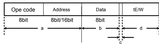
Fig.48 WRITE cancel valid timing
