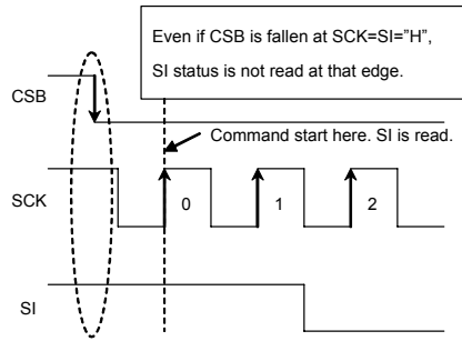
Fig.43 Operating timing
