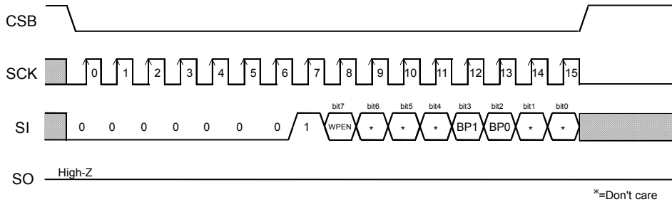
Fig.40 Status register write command (BR25H080/160/320-W)
