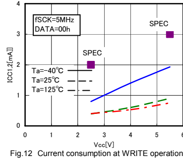
Fig.12 Current consumption at WRITE operation ICC_{1,2}
