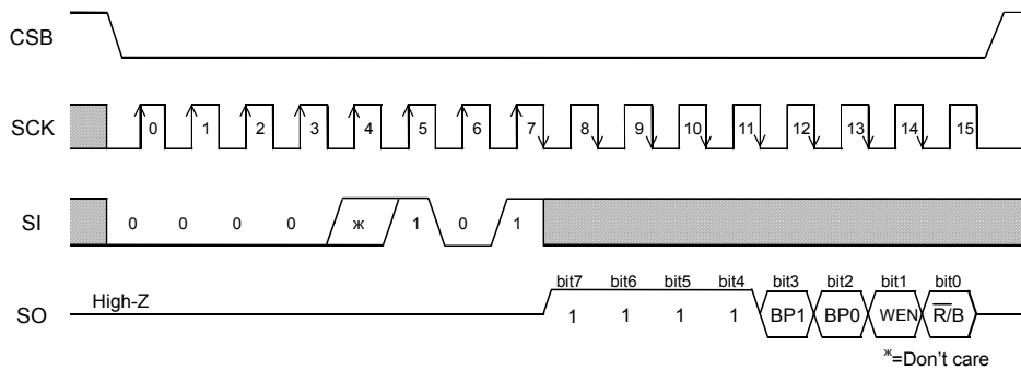
Fig.41 Status register read command (BR25H010/020/040-W)
