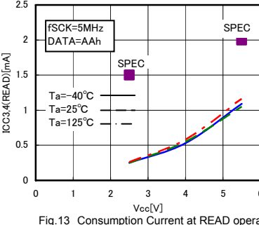
Fig.13 Consumption Current at READ operation ICC_{3,4}
