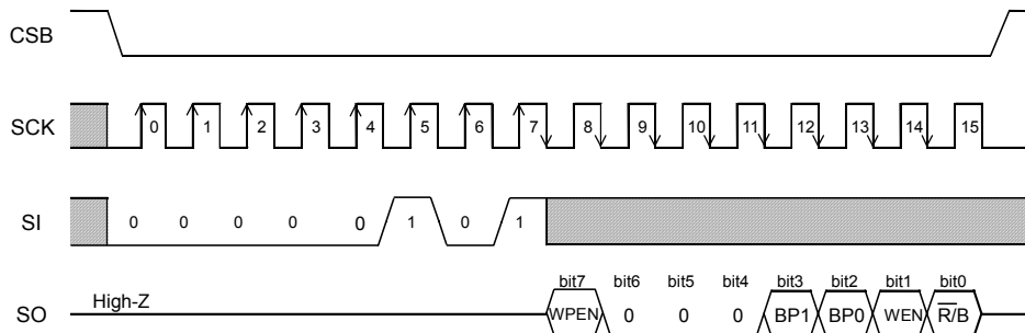
Fig.41 Status register read command (BR25H010/020/040-W)
