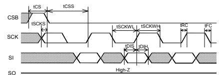
Fig.3 Input timing
