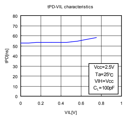
Fig.53 VIL dependency of data output delay time
