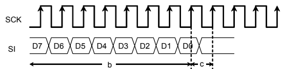
Fig.48 WRITE cancel valid timing
