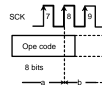
Figure 50. WREN/WRDI cancel valid timing
