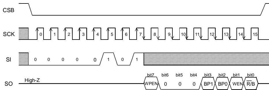
Figure 42. Status register read command
