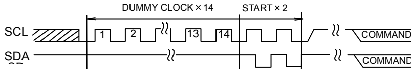
Fig. 41-(a) DUMMY CLOCK \times 14 + START+START
