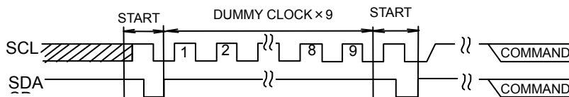
Fig. 41-(b) START + DUMMY CLOCK \times 9 + START
