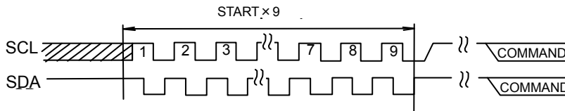
Fig. 41-(c) START \times 9
