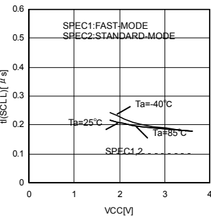
Fig.28 Noise Spike Width t(SCL L)
