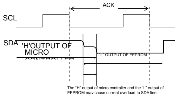
Fig.47 Input/Output Collision Timing
