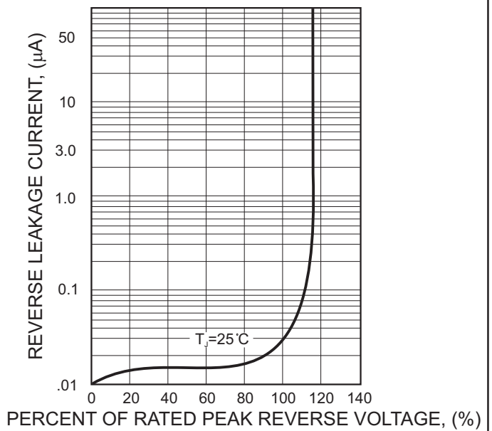
FIG.4-TYPICAL REVERSE CHARACTERISTICS
