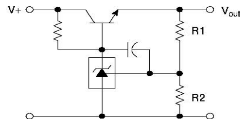
Series Pass Regulator V_{out} = \left(1 + \frac{R1}{R2}\right) V_{ref} V_{out\ min} = V_{ref} + V_{be}
