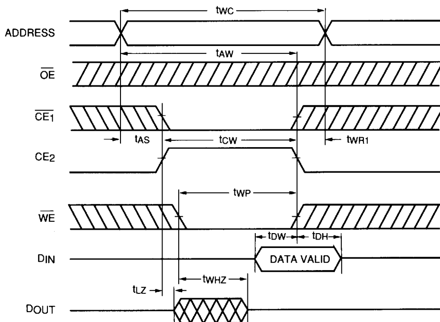
FIGURE 7. WRITE CYCLE TIMING NO. 3 ( \text{CE}_2 CONTROL)
