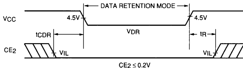
FIGURE 2. LOW V_{CC} DATA RETENTION WAVEFORM ( CE_2 CONTROLLED)
