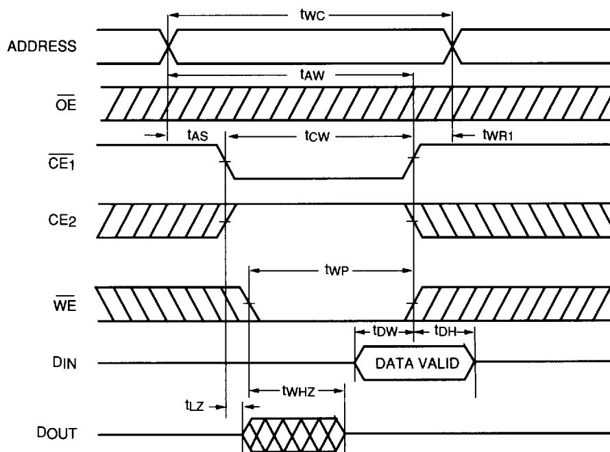
FIGURE 6. WRITE CYCLE TIMING NO. 2 ( \overline{\text{CE}}_1 CONTROL)
