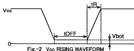
Fig.-2 Vcc RISING WAVEFORM
