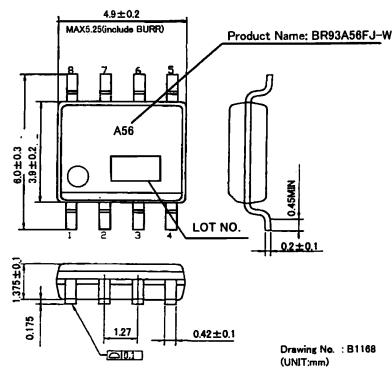
Fig-4(c) PHYSICAL DIMENSION SOP-J8 (BR93A56FJ-W)
