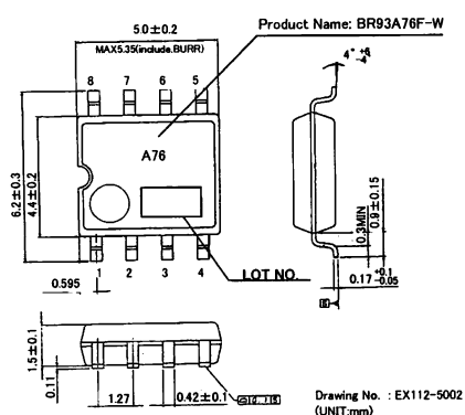
Fig-4(a) PHYSICAL DIMENSION SOP8 (BR93A76F-W)
