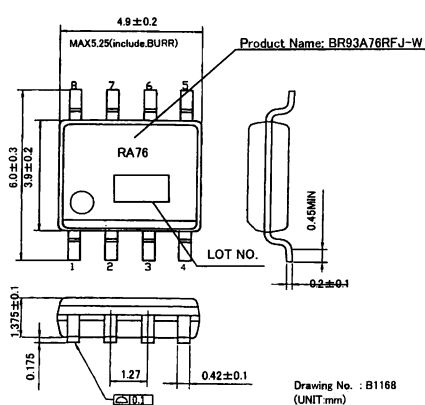
Fig-4(d) PHYSICAL DIMENSION SOP-J8 (BR93A76RFJ-W)
