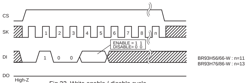
Fig.33 Write enable / disable cycle
