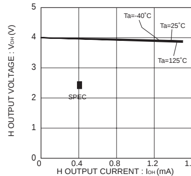
Fig.7 H output voltage V_{OH-IOH} ( V_{CC} = 4.0\text{V} )
