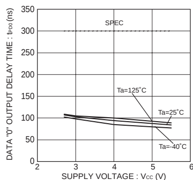
Fig.23 Data "0" output delay time t_{PD0}
