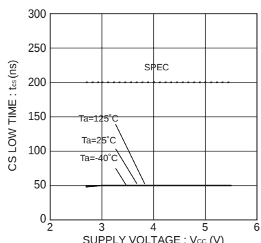
Fig.17 CS low time t_{CS}
