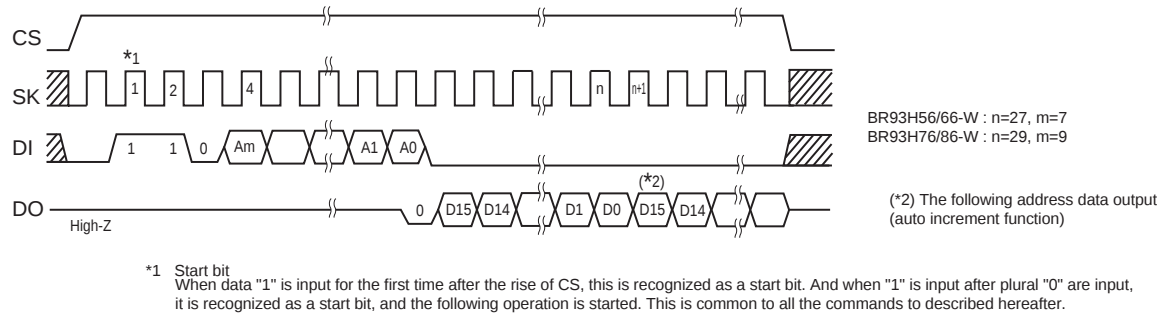
Fig.30 Read cycle
