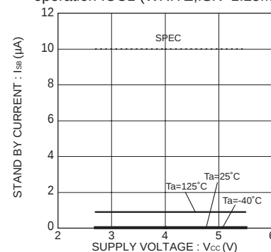
Fig.13 Consumption current at standby operation I_{SB}
