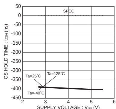
Fig.21 CS hold time t_{CSH}
