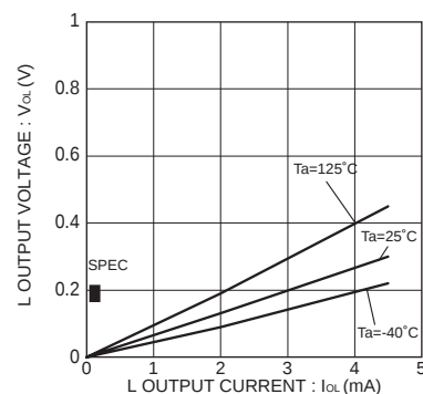
Fig.4 L output voltage V_{OL-IOL} ( V_{CC} = 2.7\text{V} )
