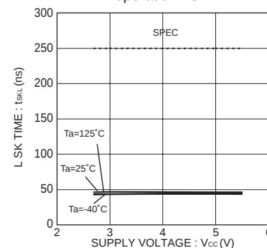
Fig.16 SK low time t_{SKL}
