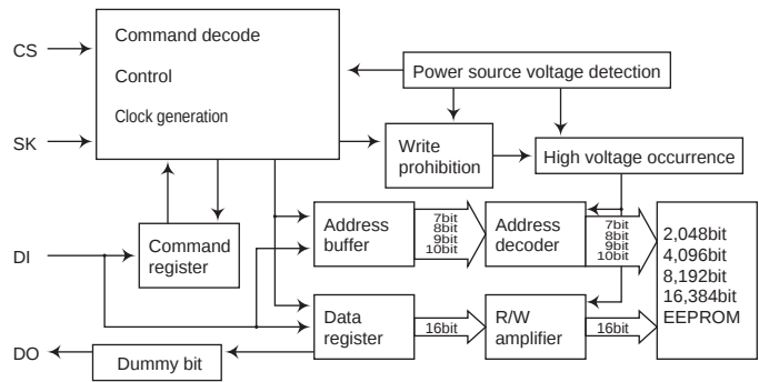
Fig.27 Block diagram
