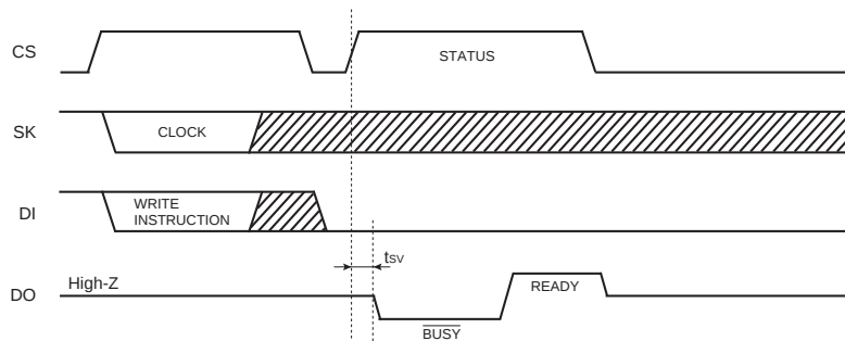
Fig.45 R/\overline{B} status output timing chart
