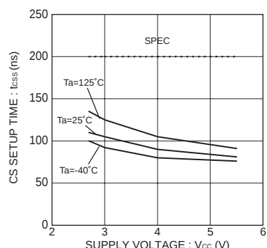
Fig.18 CS setup time t_{CSS}
