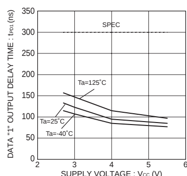
Fig.22 Data "1" output delay time t_{PD1}
