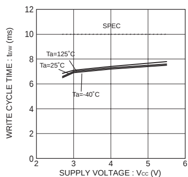
Fig.26 Write cycle time t_{E/W}
