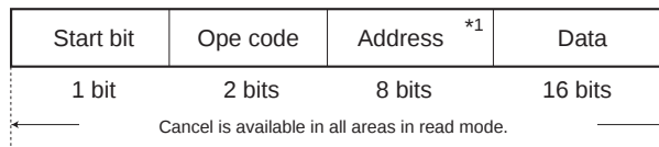
Fig.34 READ cancel available timing
