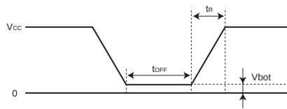
Fig.52 Rise waveform diagram
