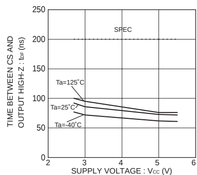
Fig.25 Time from CS to High-Z t_{DF}
