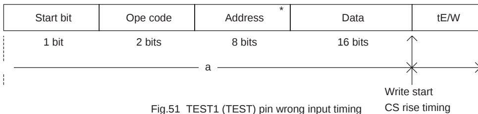
Fig.51 TEST1 (TEST) pin wrong input timing CS rise timing
