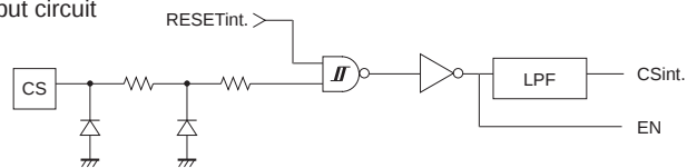
Fig.37 CS input equivalent circuit
