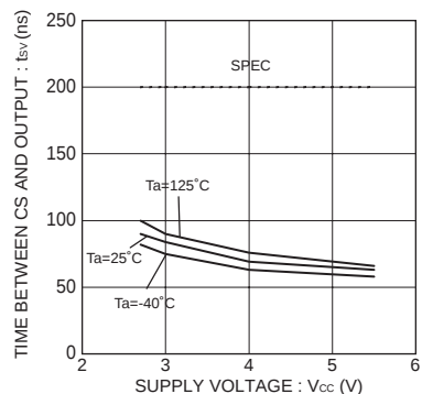
Fig.24 Time from CS to output establishment t_{SV}
